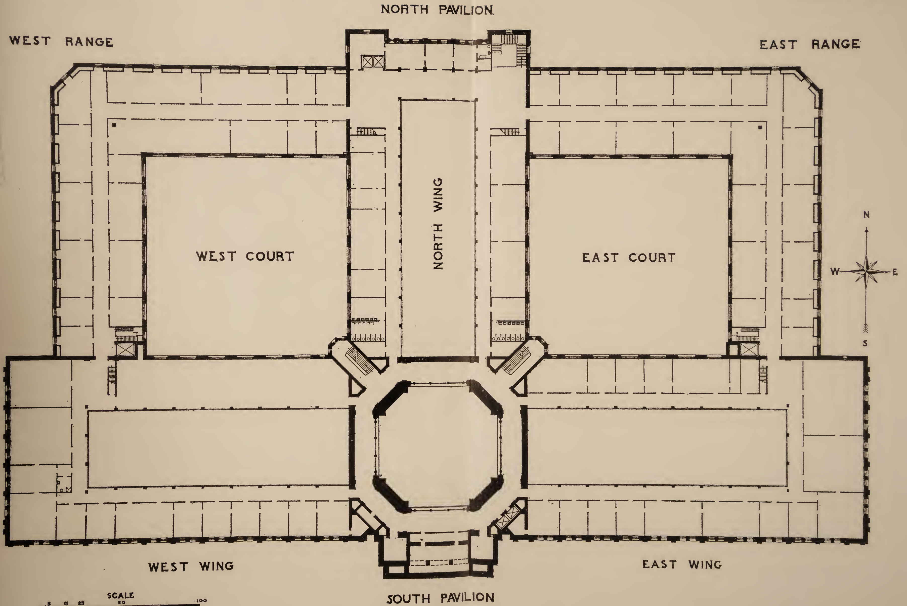
PLAN OF THIRD STORY.
